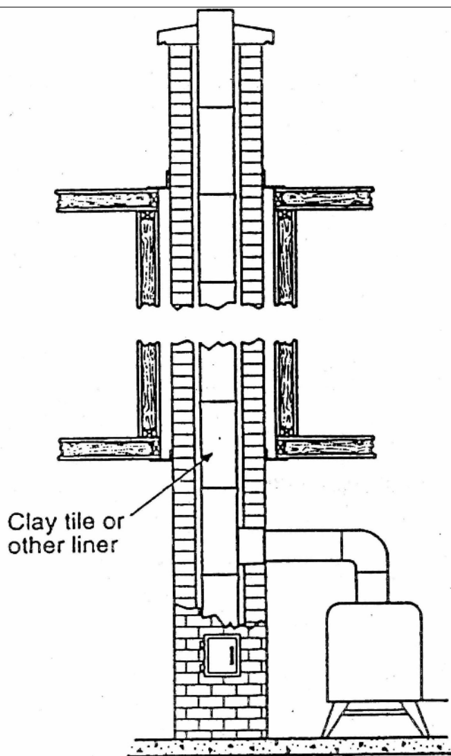
Masonry chimney
