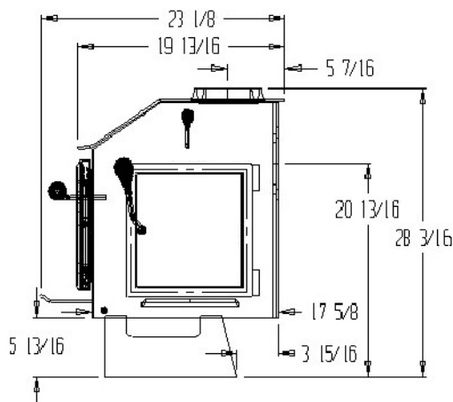
S8000II Side Dimensions
