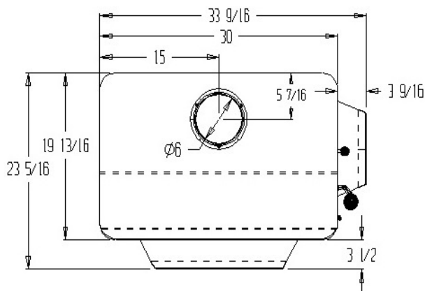
S8000II Top Dimensions
