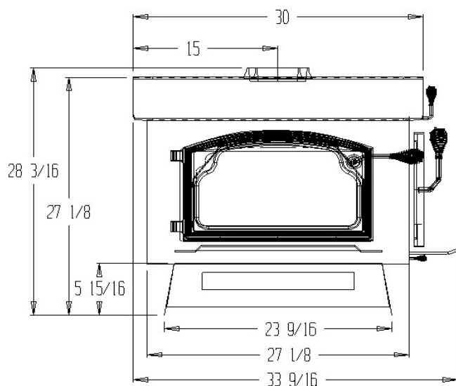
S8000II Front Dimensions
